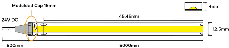
End Cap Product Code-COB-CAP
